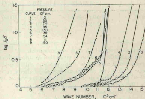
FIG. 11. Log I_0/I versus wave number for gallium arsenide.
